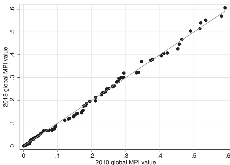
Figure 10. Quintile-Quintile Plot: Global Distributions of MPI
