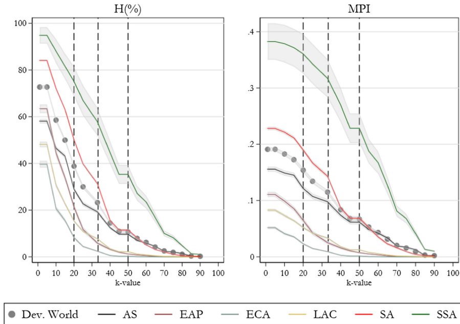
Figure 6. Complementary Cumulative Distribution Functions of H and MPI by World Region Notes: (a) AS: Arab States; EAP: East Asia and the Pacific; ECA: Europe and Central Asia; LAC: Latin America and the Caribbean; SA: South Asia; SSA: Sub-Saharan Africa. (b) Gray-shaded regions represent 95 percent confidence intervals.
